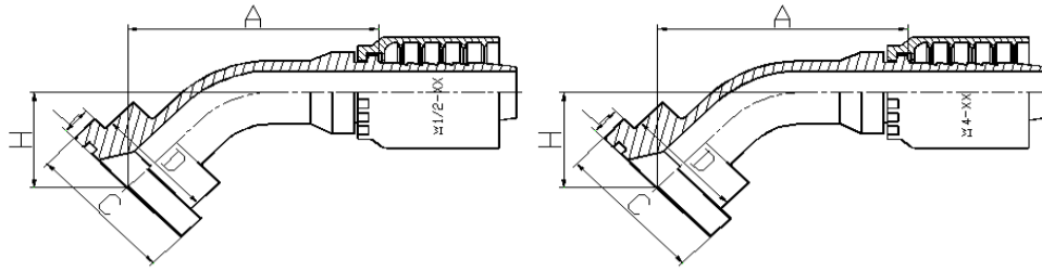
45° FLANGE S SERIES / CODE 62
