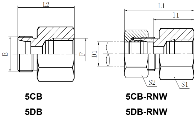
METRIC MALE 24° CONE/BSP FEMALE STUD FITTINGS
