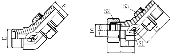
45° ELBOW METRIC MALE 24° CONE / ADJUSTABLE METRIC MALE ORING SEAL
