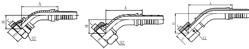
45° ORFS FEMALE FLAT SEAT
