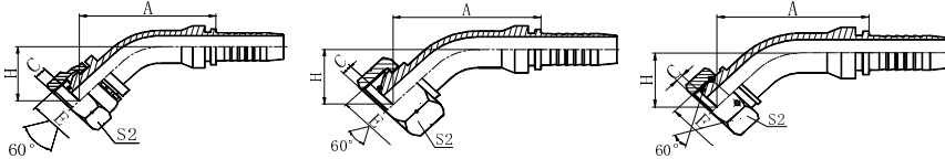
° BSP FEMALE 60° CONE WITH O-RING
